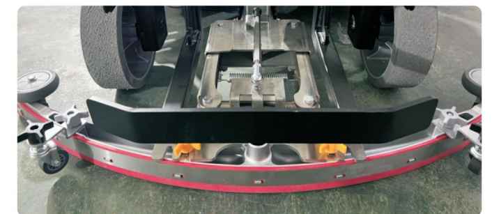
10 The wiper connecting rod structure is not easy to deform
